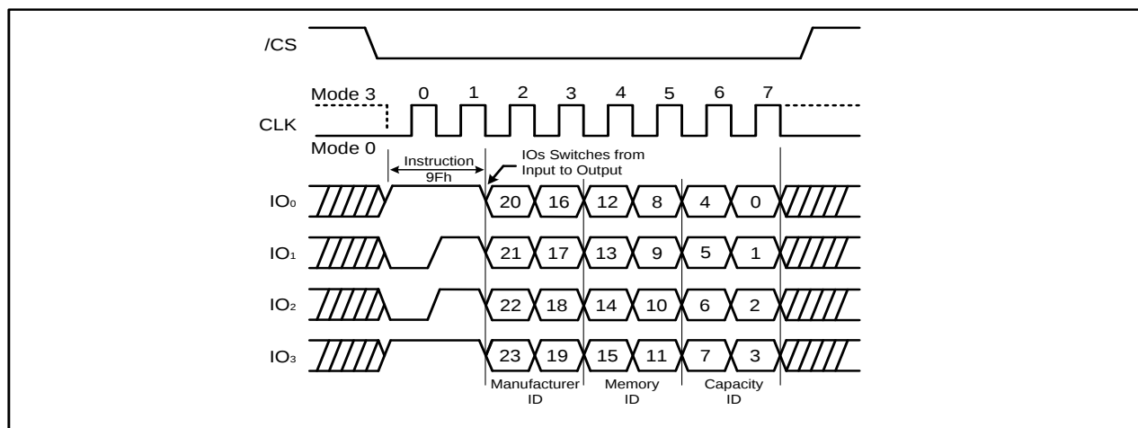
Figure 37b. Read JEDEC ID Instruction (QPI Mode)
